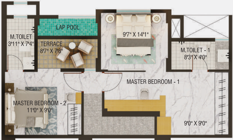
▼ TYPICAL UPPER LEVEL UNIT PLAN
